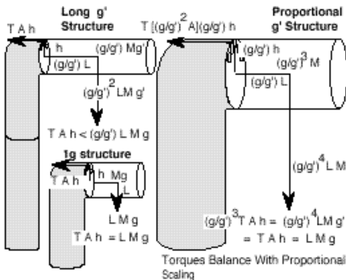
Figure 7. Ultrasaurus scaled to various surface gravities.
