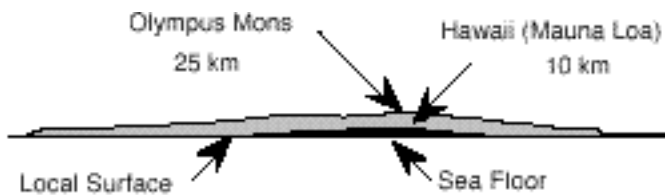
Fig. 5 Slopes and Elevation of Olympus Mons and Hawaii
