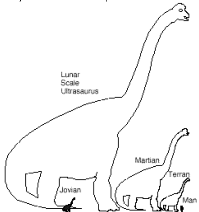
Figure 7. Ultrasaurus scaled to various surface gravities.
